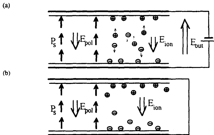
Fig.6 The inverted bistability model for a SSFLC Cell with alignment layer:
